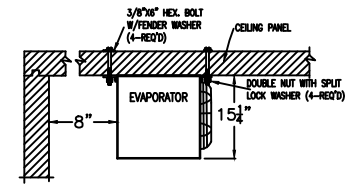
EVAPORATOR MOUNTING DETAIL
