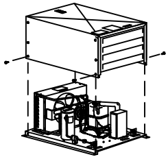
CONDENSING UNIT DETAIL
