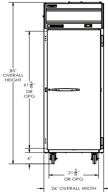
ELEVATION VIEW
