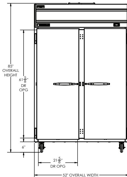
ELEVATION VIEW
