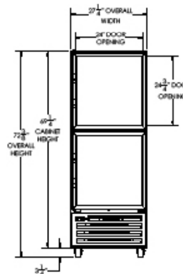
ELEVATION VIEW
