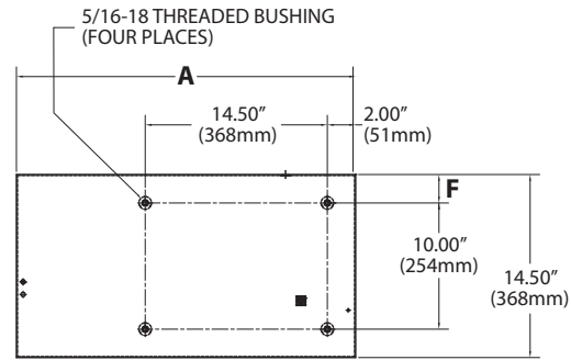
BASE MOUNTING DETAIL
