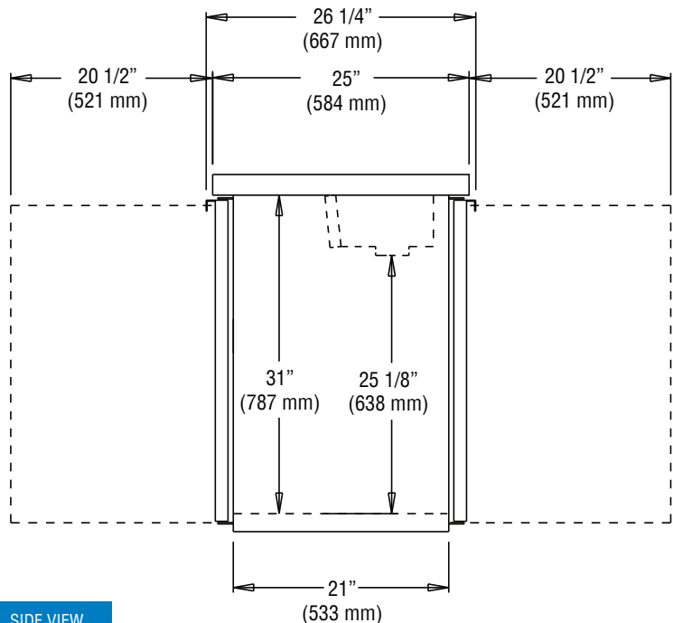
SIDE VIEW
