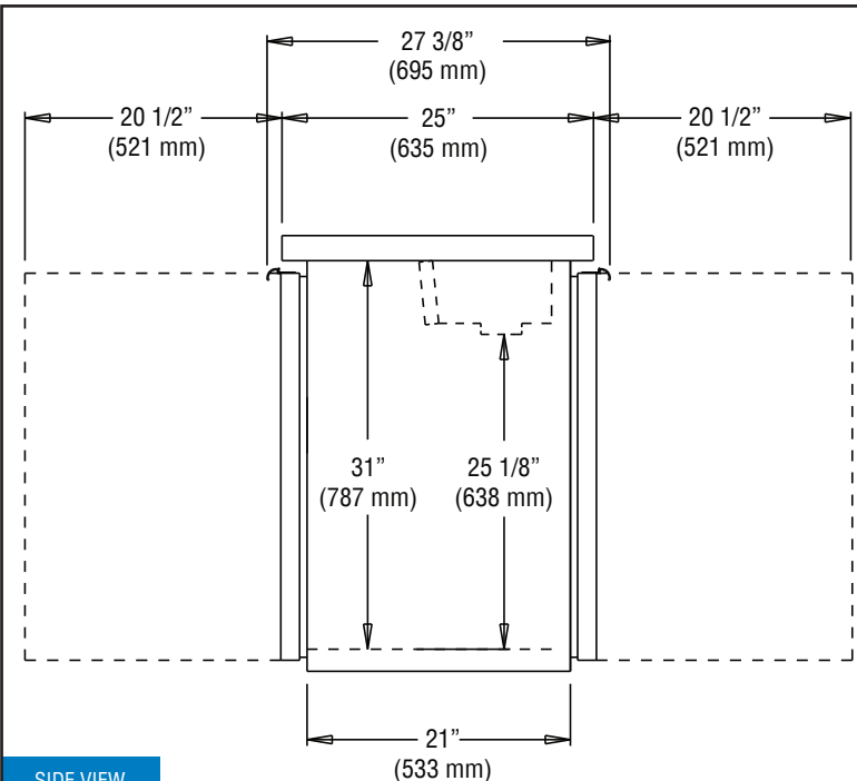
SIDE VIEW
