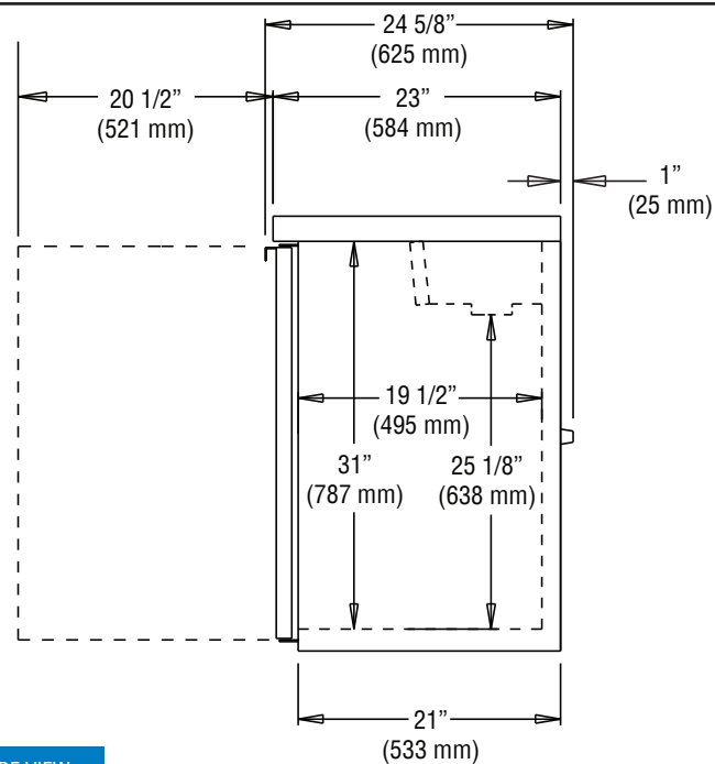
SIDE VIEW
