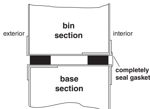
Cross section of ITS sections joined
