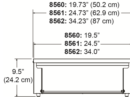
Operator View
