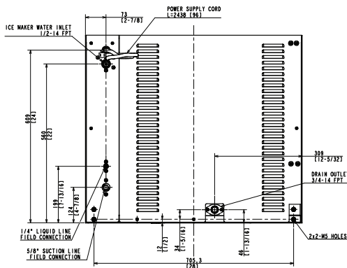
REMOTE AIR-COOLED
