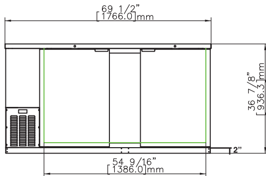
HBB-3G-LD-69(-S) Front View
