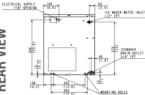
AIR-COOLED
