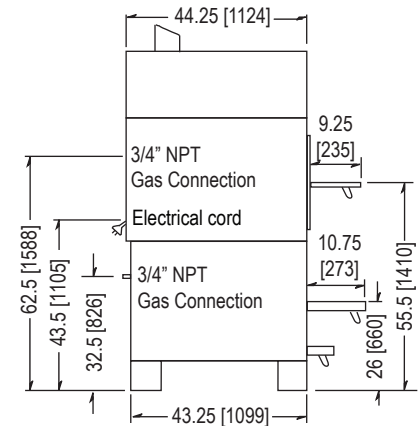
SIDE VIEW - MBC 1048 / MBC 1060
