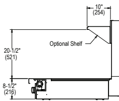
SIDE VIEW of MODULAR MODEL
