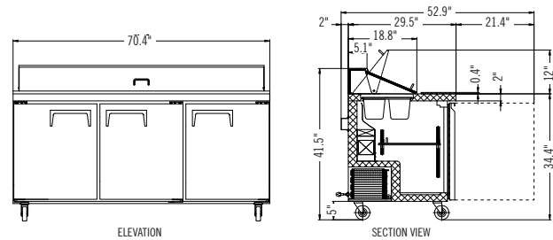
VALSL-3D
