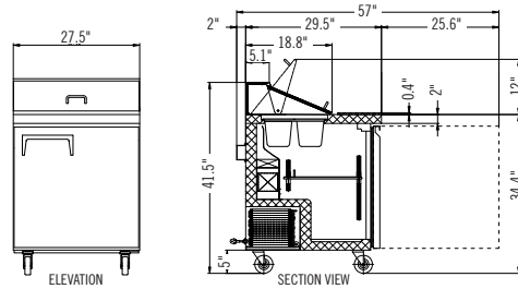
VALSL-1D
