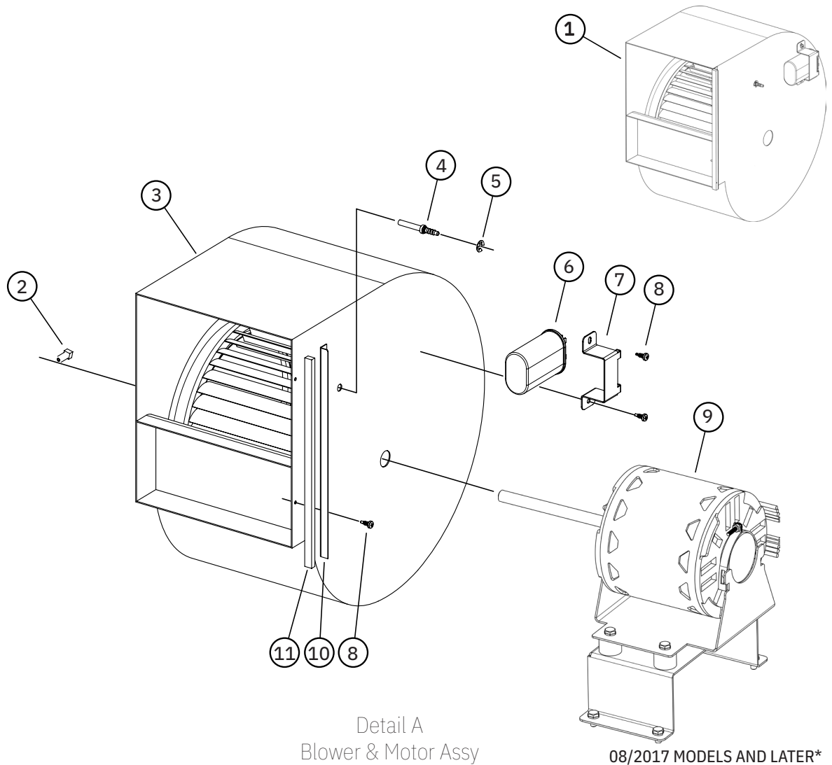
DETAIL A, Blower & Motor Assy
